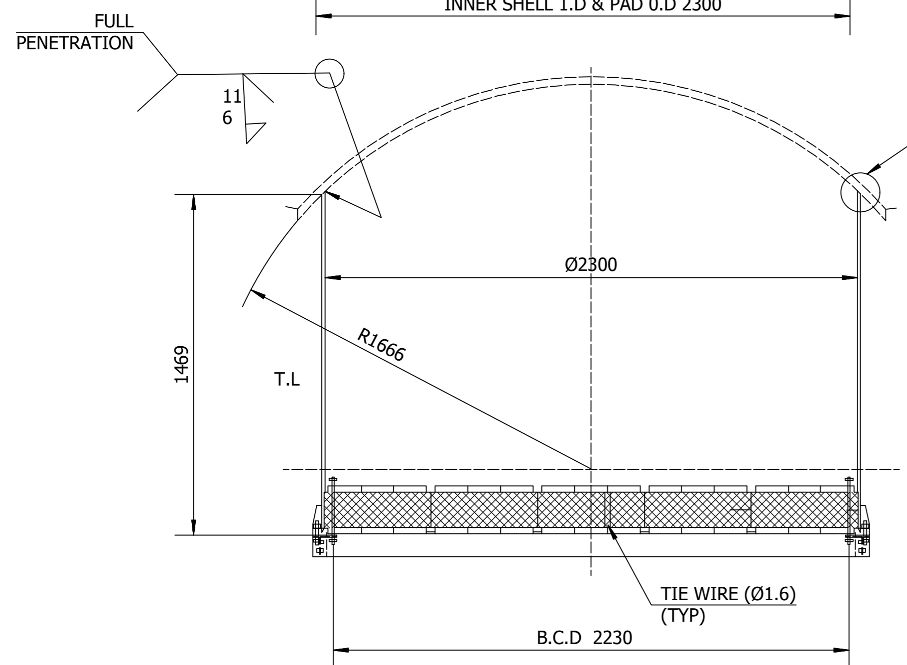
PLAN VIEW OF DEMISTER
